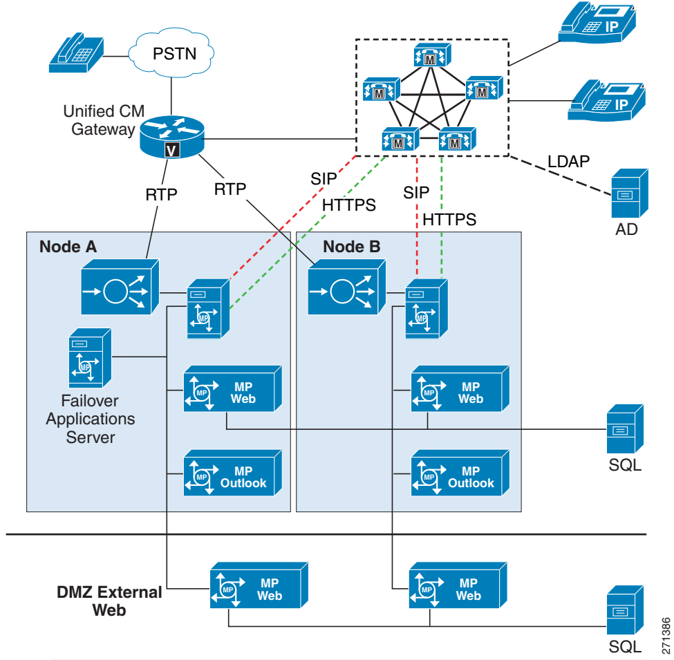
Figure 14-2 Reservationless Single-Number Access Deployment
