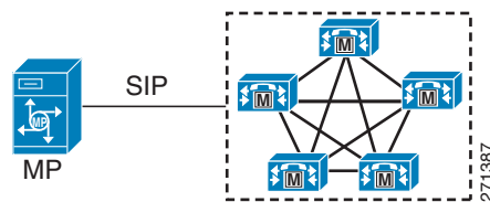
Figure 14-3 SIP Integration with Unified CM
