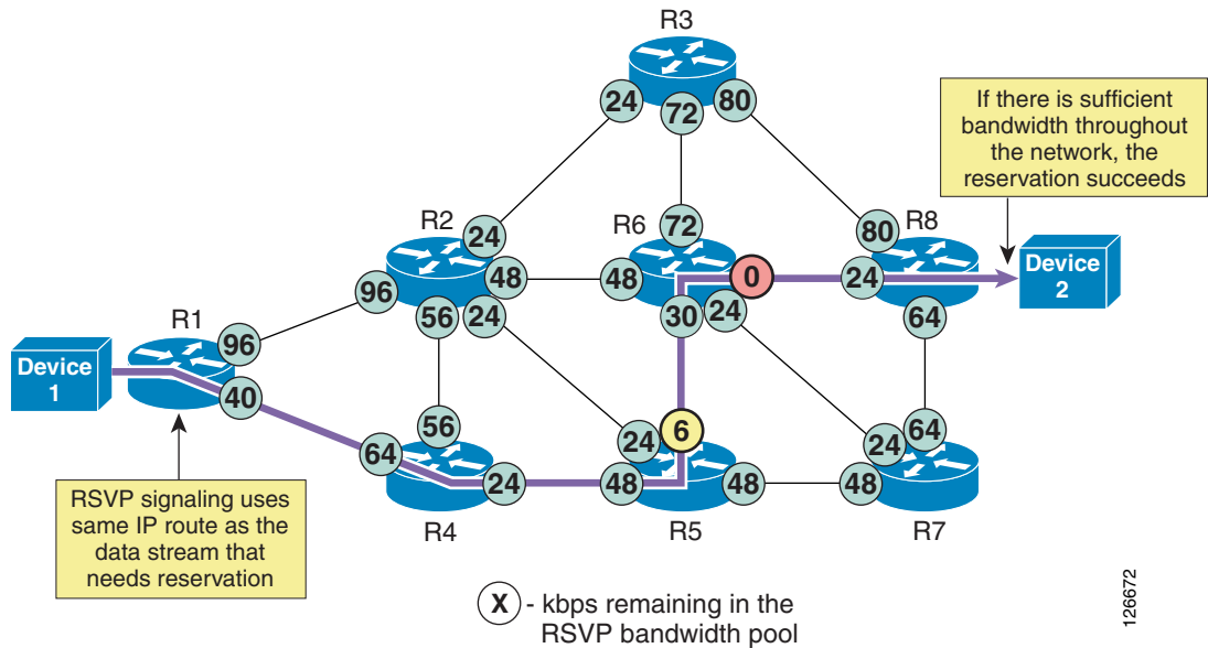
Figure 9-7 RSVP Signaling for a Successful Reservation
