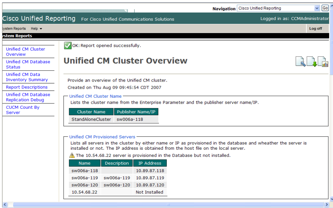
Figure 1 User Interface
