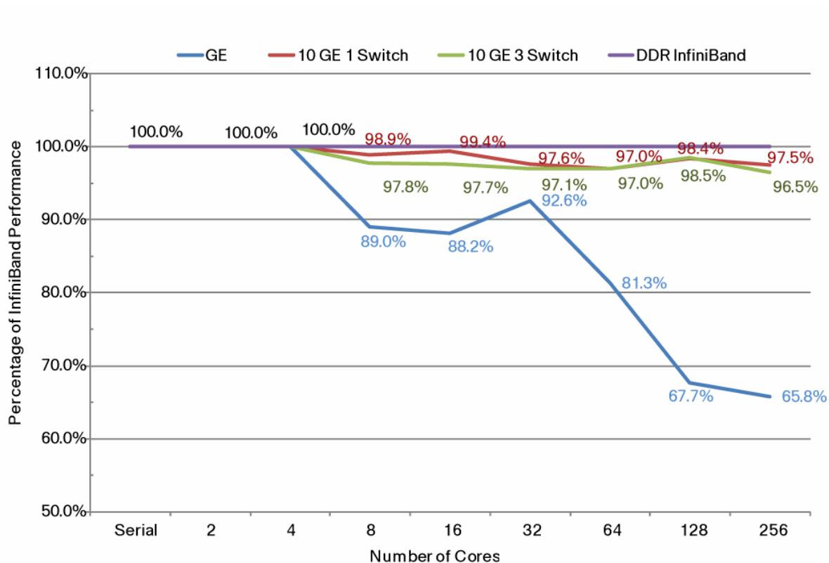
Figure 2. Speed Up as a Percentage of InfiniBand Performance
