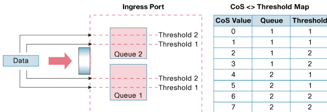
Figure 6. Mapping a Packet to a Queue or Threshold
