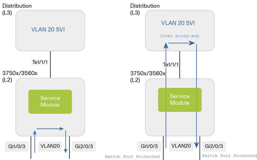
Figure 2. How to Monitor Locally Switched Traffic (Left) with Private VLAN (Right) for Layer 2 Configured Switch or Stack
