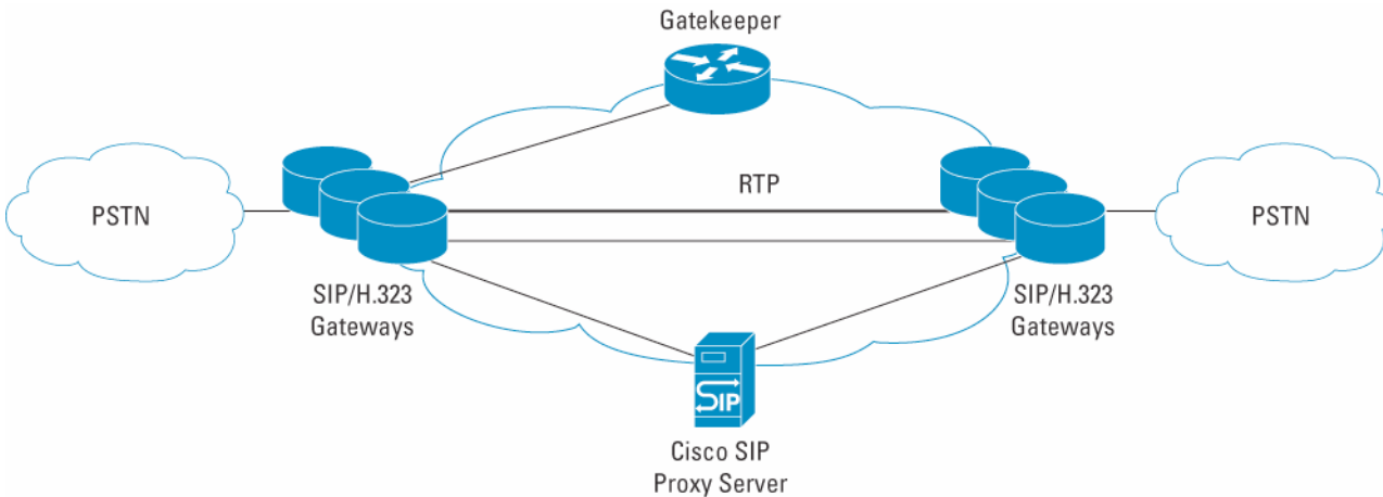
Figure 1. SIP and H.323 Wholesale Call Transport
