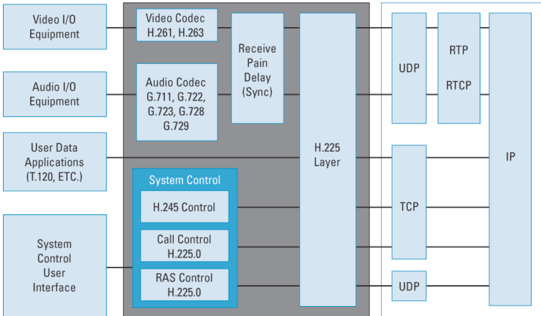
Figure 2. H.323 Protocol Suite Overview
