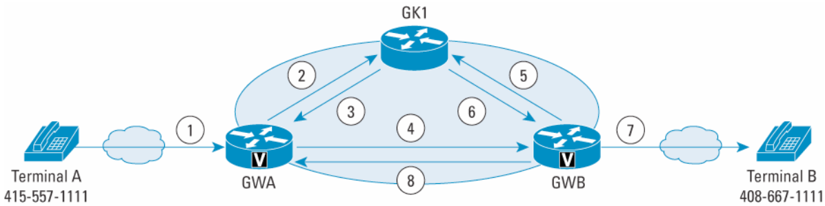
Figure 4. Intra-Zone Call Message Sequence
