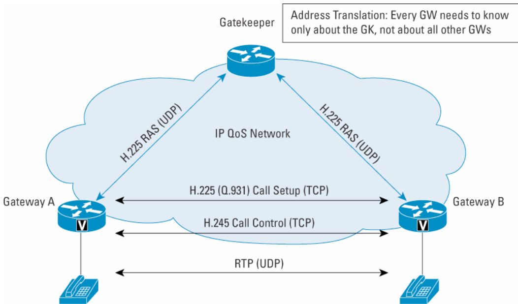
Figure 3. Basic Constituents of a H.323 Call
