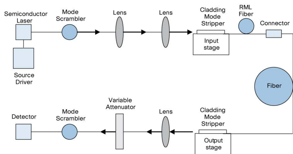
Figure 5. RML Bandwidth Measurement Test Setup
