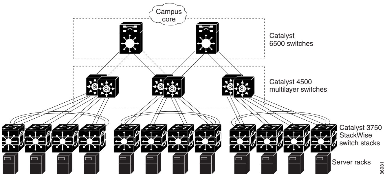
Figure 1-4 Server Aggregation
