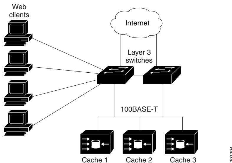
Figure 41-1 Cisco Cache Engine and WCCP Network Configuration
