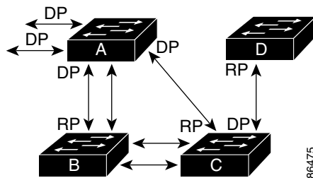
Figure 15-3 Spanning-Tree Topology
