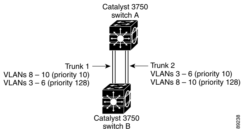
Figure 10-3 Load Sharing by Using STP Port Priorities
