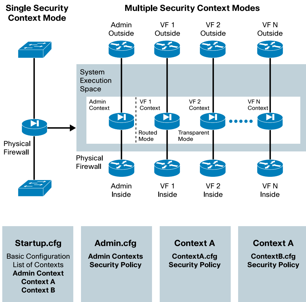
Figure 6. Virtualized Firewall
