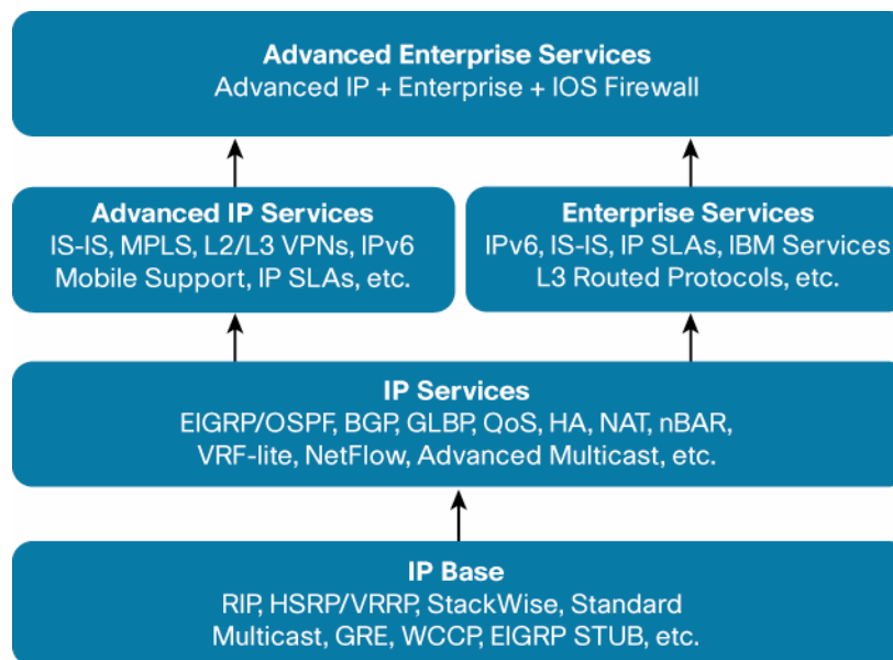
Figure 1. Cisco IOS feature set map up to 12.2(18)SXF
