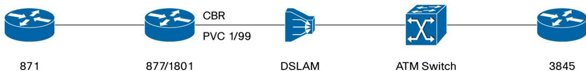
Figure 7. Deploying Cisco ISR with an External DSL Modem
