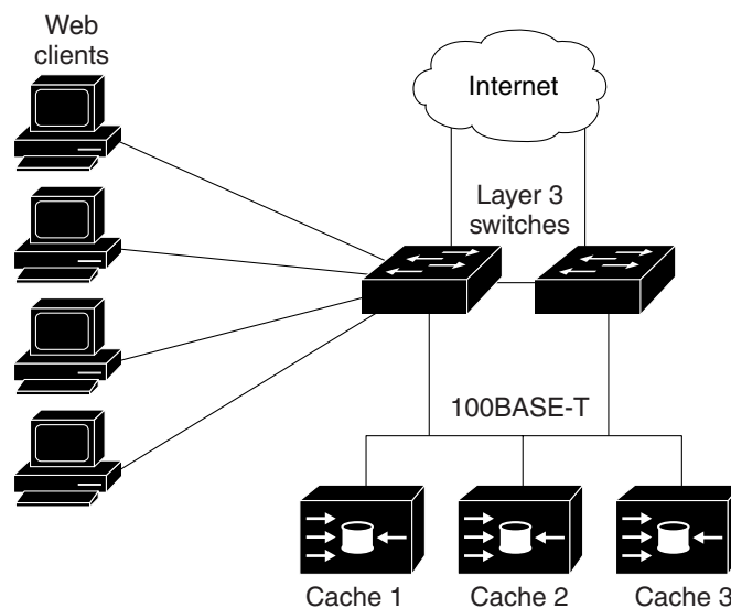
Figure 42-1 Cisco Cache Engine and WCCP Network Configuration
