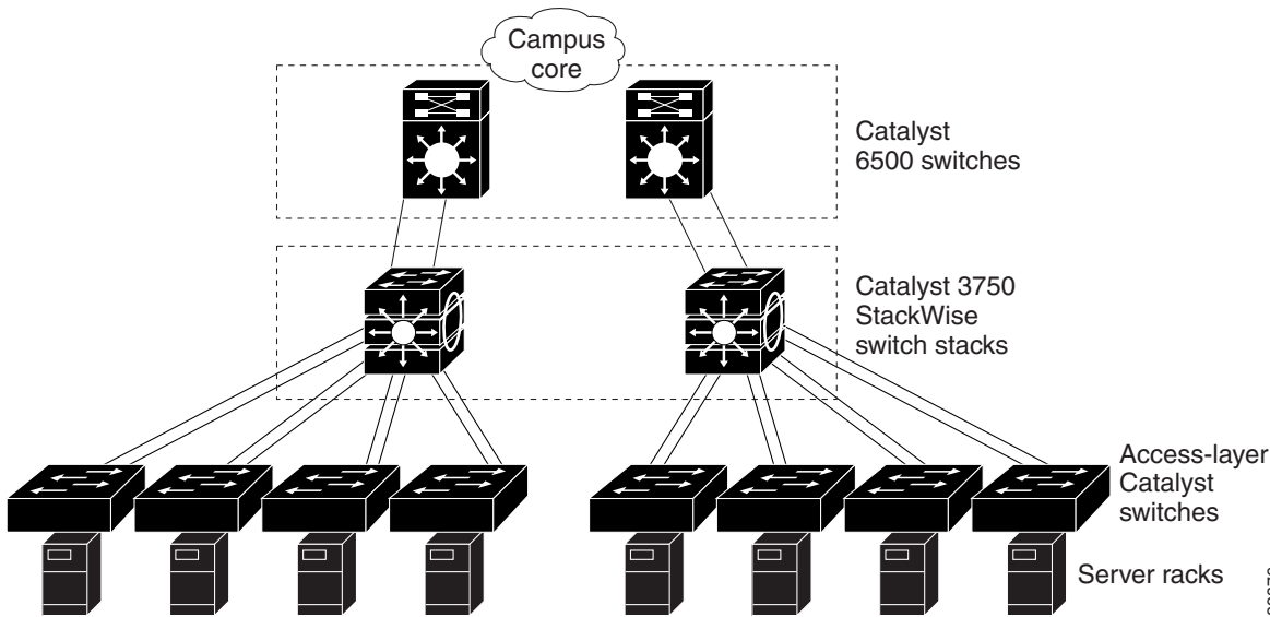
Figure 1-2 Server Aggregation
