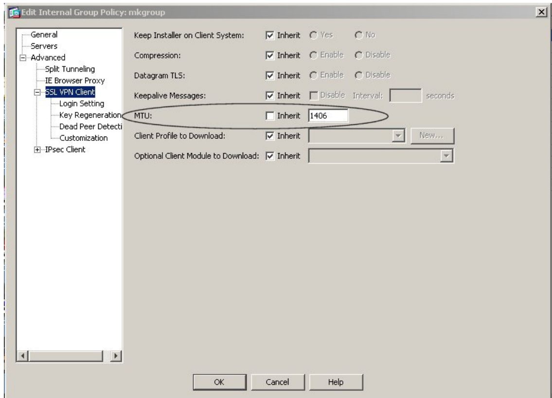
Figure 9-1 Edit Internal Group Policy Dialog Box
