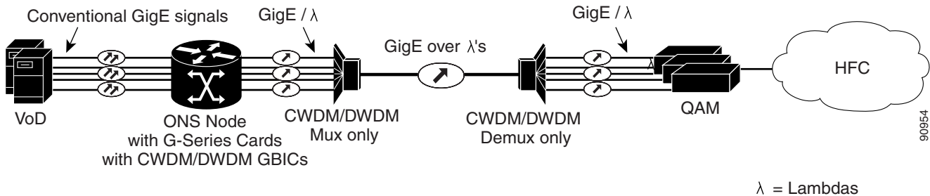
Figure 5-11 G-1K-4 with CWDM/DWDM GBICs in Cable Network
