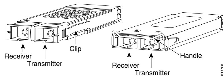
Figure 5-9 GBICs with Clips (left) and with a Handle (right)
