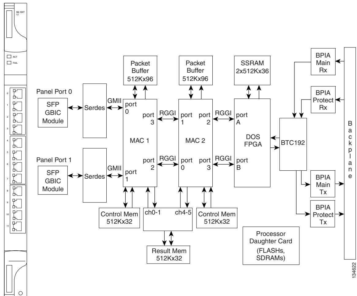
Figure 5-6 ML100X-8 Faceplate and Block Diagram
