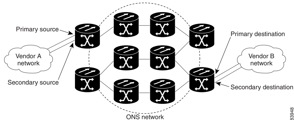
Figure 10-4 Secondary Sources and Drops
