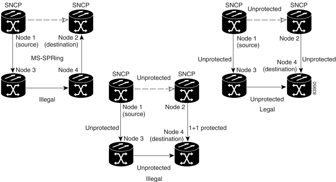
Figure 10-6 Mixing 1+1 or MS-SPRing Protected Links with an SNCP
