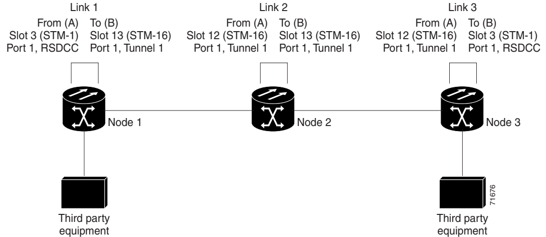
Figure 10-1 DCC Tunnel
