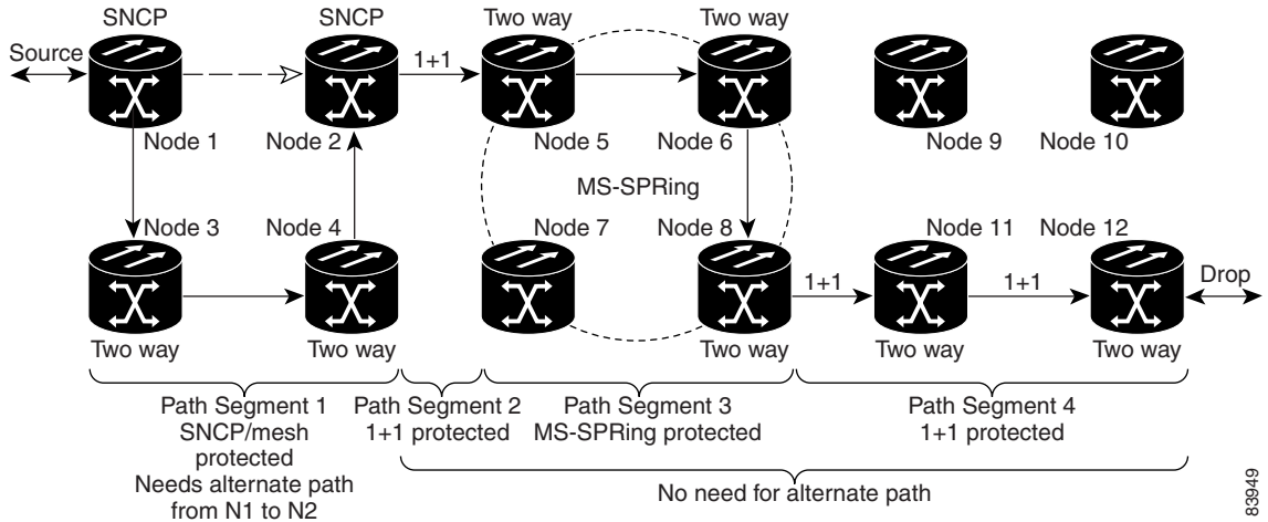
Figure 10-5 Alternate Paths for Virtual SNCP Segments
