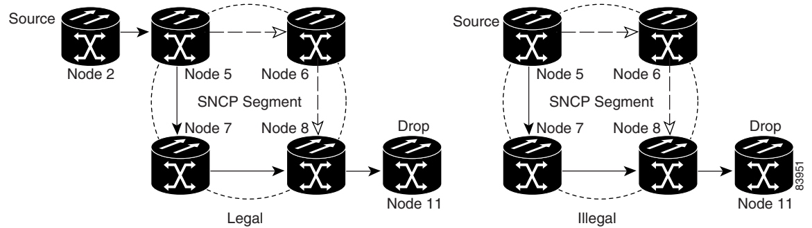
Figure 10-8 Ethernet and SNCP
