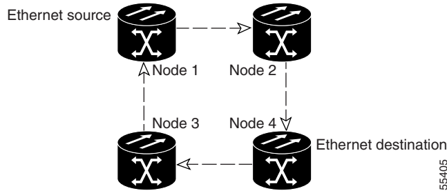
Figure 10-7 Ethernet Shared Packet Ring Routing
