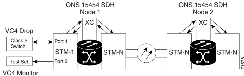
Figure 10-2 VC4 Monitor Circuit Received at an STM-1 Port
