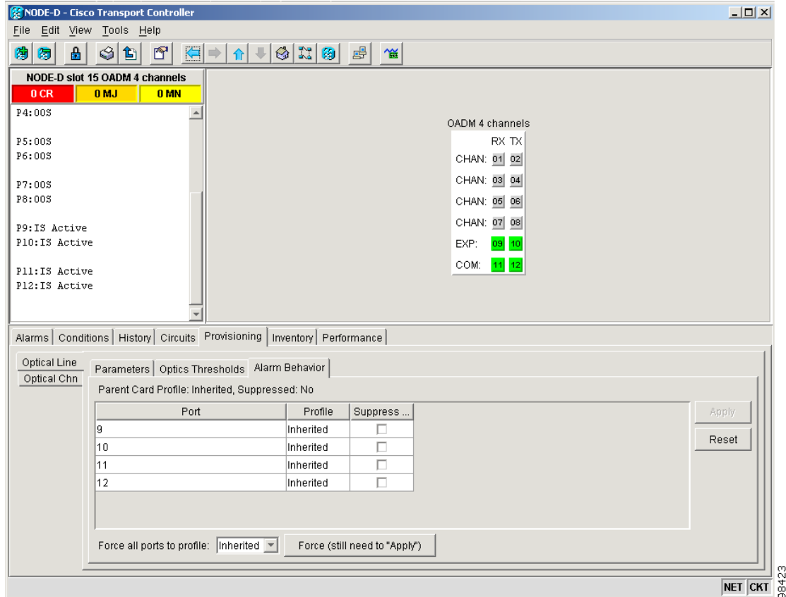
Figure 14-4 Card View Port Alarm Profile for an AD-4C-xx.x Card
