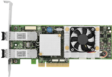
Broadcom NetXtreme II BCM57711 Dual-Port 10 GbE PCIe Adapter Card with TOE and iSCSI HBA
