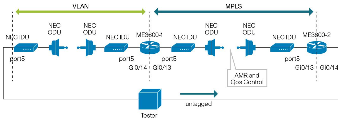
Figure 16: Testing of End-to-End Connection
