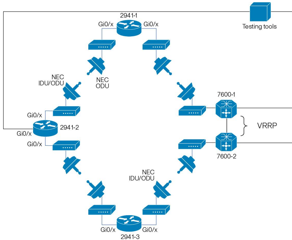
Figure 17: Testing of Transport Protection
