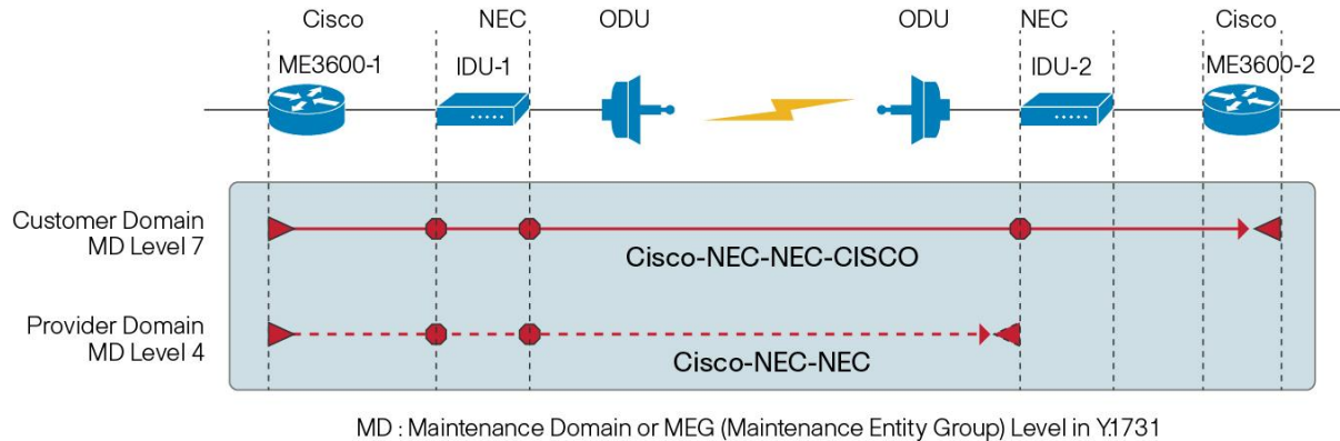
Figure 15: Ethernet OAM End-to-End Interoperability Testing
