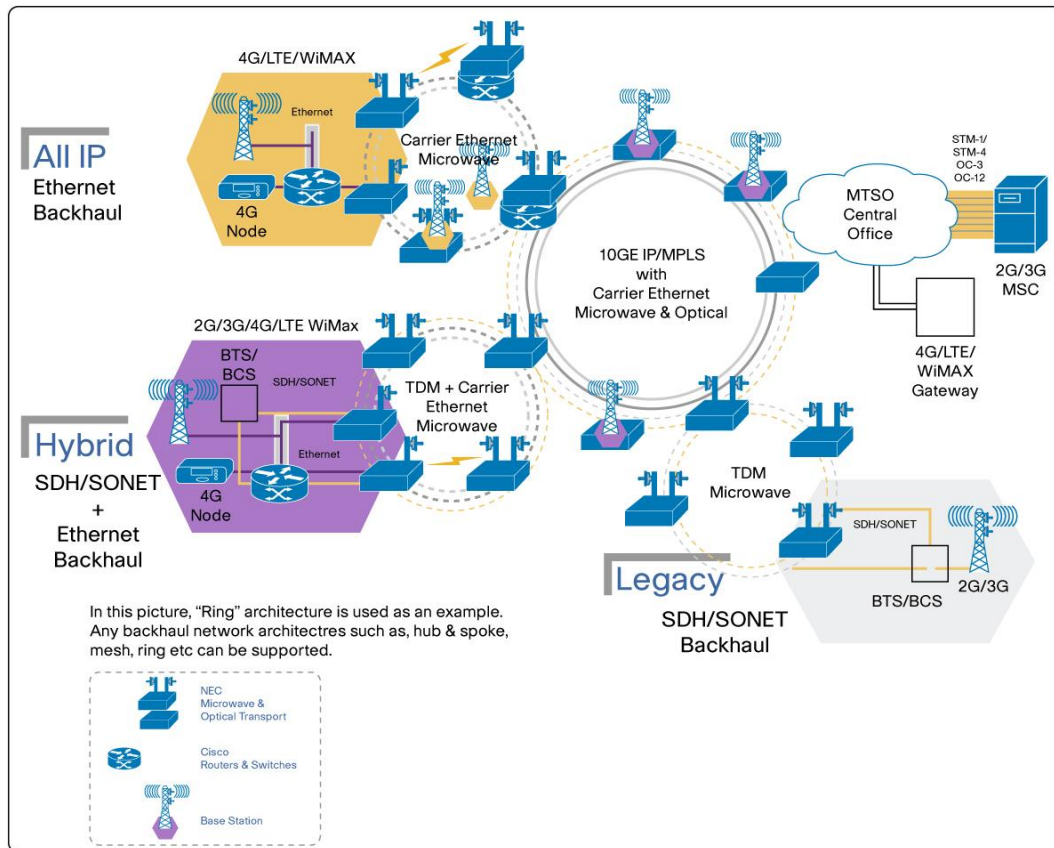
Figure 12: Converged Multiservice Aggregation Network
