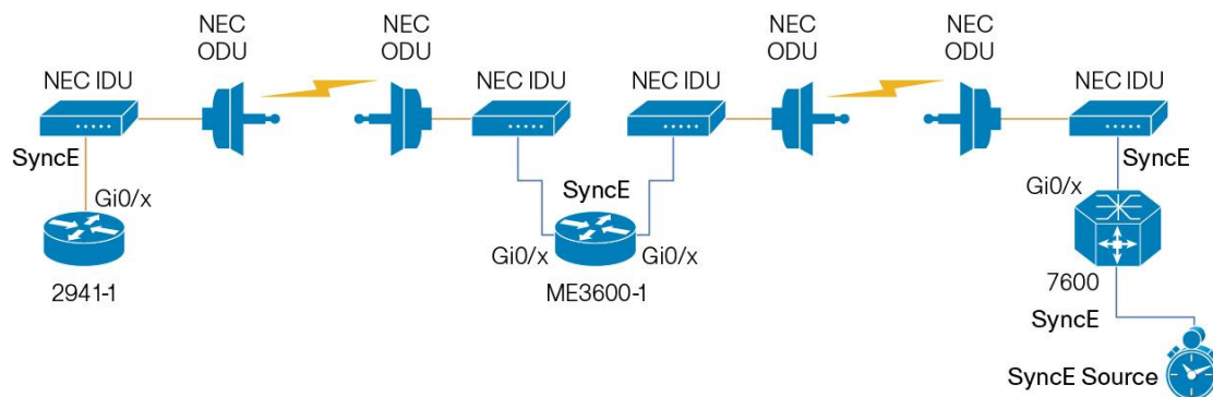
Figure 14: SyncE Interoperability Testing
