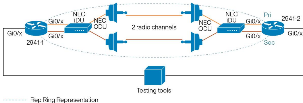
Figure 18: Testing of High-Capacity Radio
