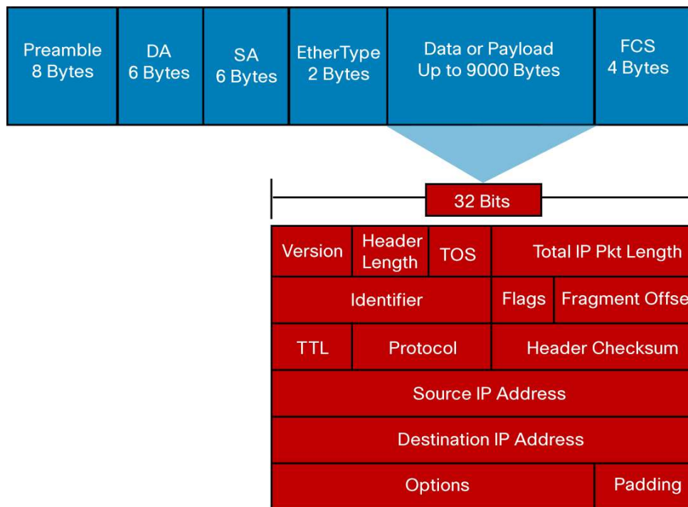
Figure 3. A Cut-Through Forwarding Decision is made as soon as enough bytes are received by the switch to make the appropriate decision
