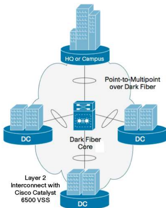
Figure 5. Data Center Interconnect through Cisco Catalyst 6500 VSS or vPC Technology
