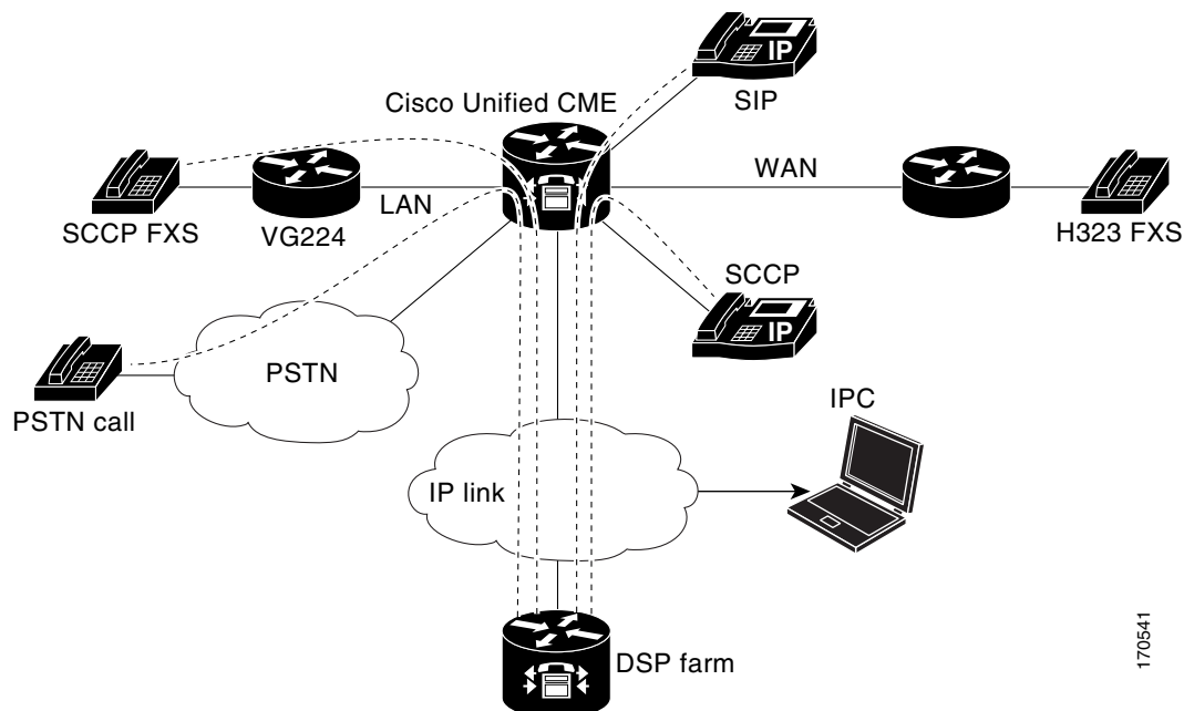
Figure 27 Cisco Unified CME and the DSP Farm on Different Routers
