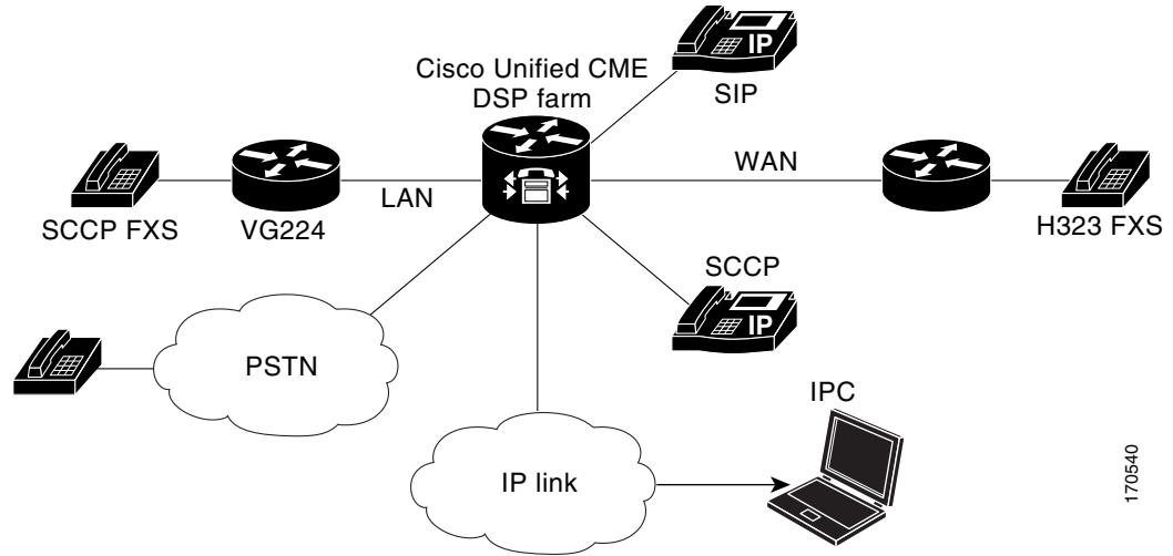
Figure 26 CME and the DSP Farm on the Same Router
