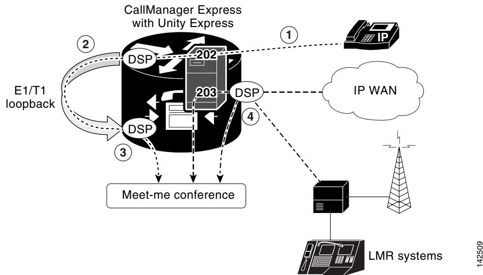
Figure 25 Meet-Me Conference in Cisco CME 3.2 to Cisco Unified CME 4.0
