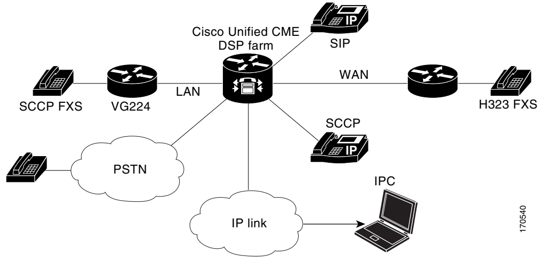
Figure 51 CME and the DSP Farm on the Same Router
