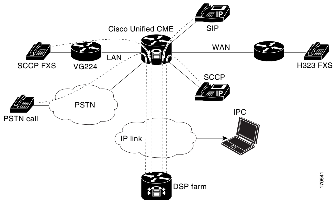
Figure 52 Cisco Unified CME and the DSP Farm on Different Routers
