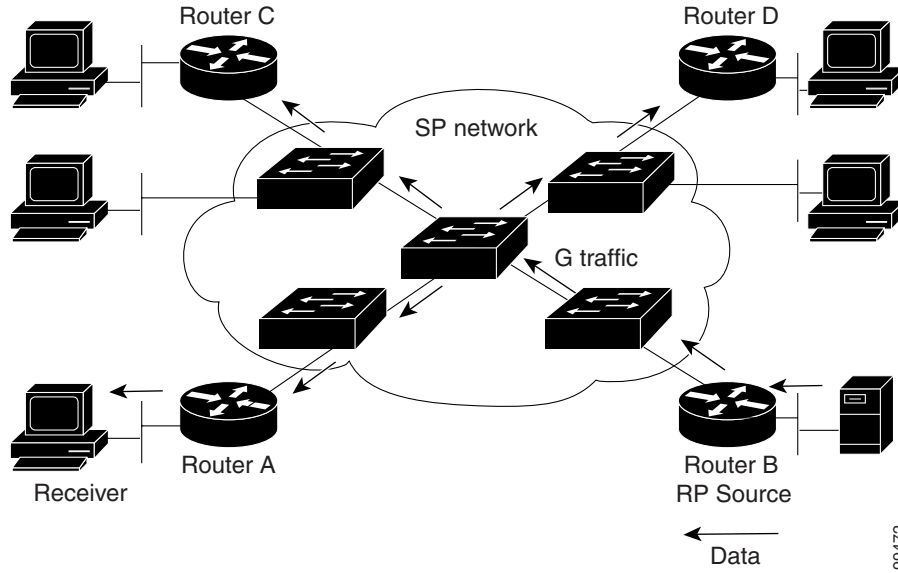
Data Traffic Flow without PIM Snooping
