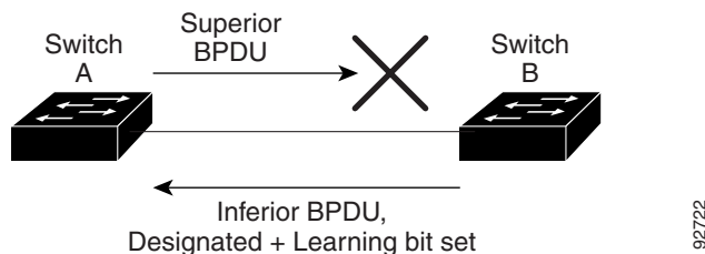
Figure 23-12 Detecting Unidirectional Link Failure
