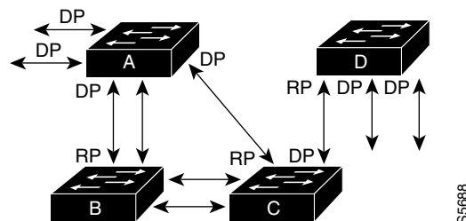
Figure 23-1 Spanning Tree Topology
