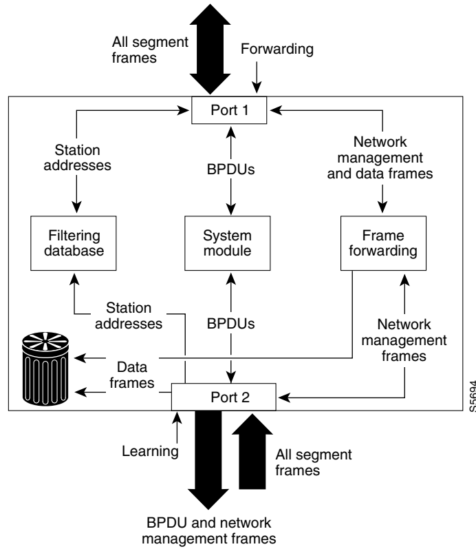
Figure 23-5 Interface 2 in Learning State
