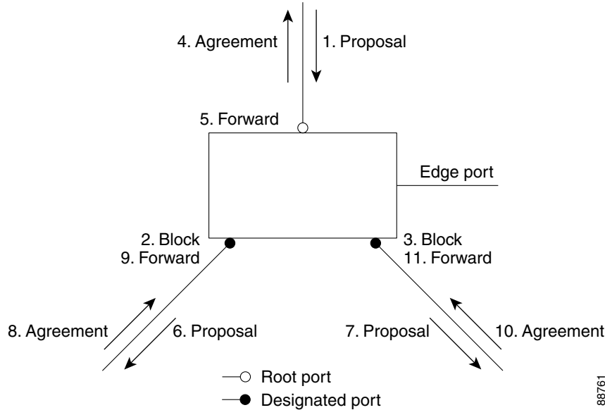
Figure 23-9 Sequence of Events During Rapid Convergence
