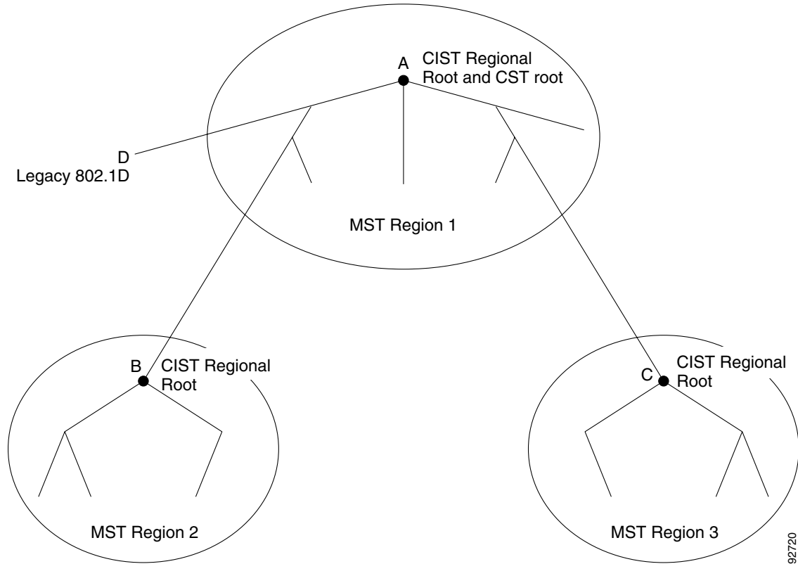
Figure 23-10 MST Regions, CIST Regional Roots, and CST Root
