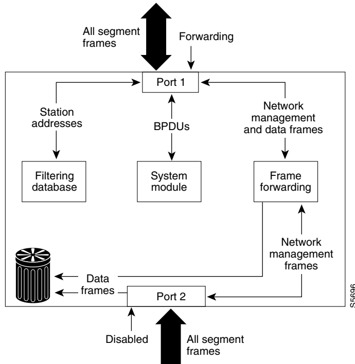
Figure 23-7 Interface 2 in Disabled State
