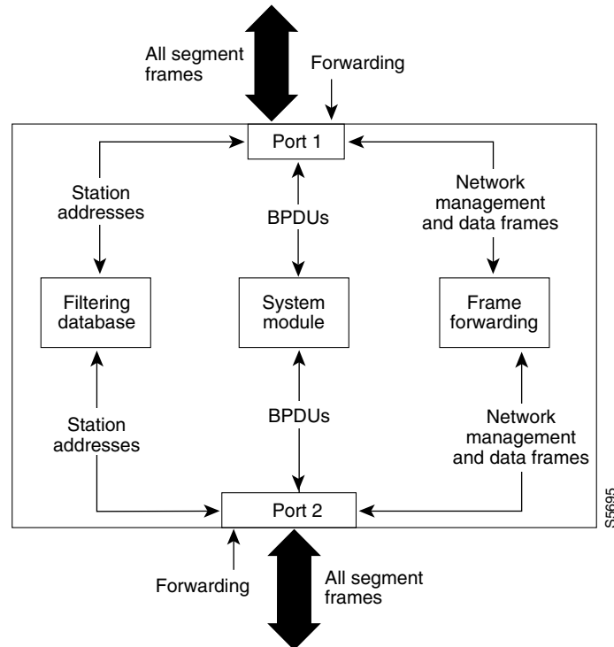
Figure 23-6 Interface 2 in Forwarding State
