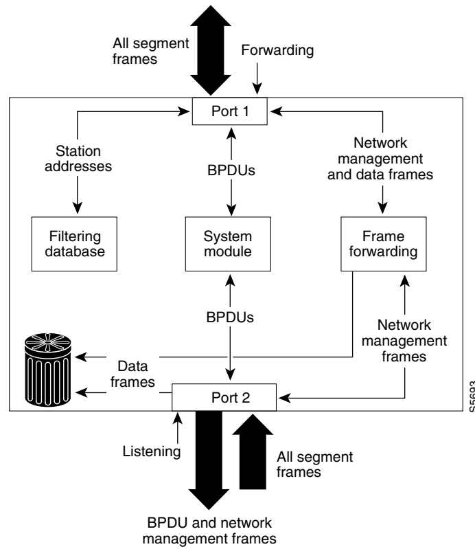
Figure 23-4 Interface 2 in Listening State
