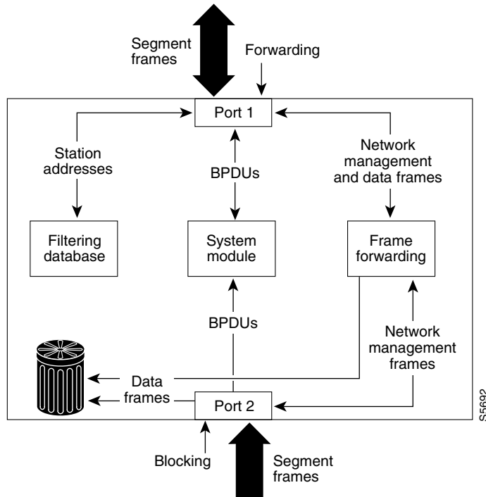
Figure 23-3 Interface 2 in Blocking State
