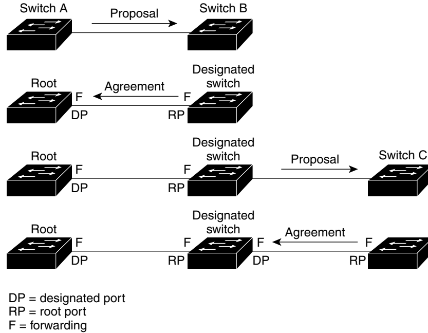
Figure 23-8 Proposal and Agreement Handshaking for Rapid Convergence
