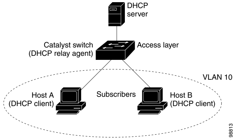
Figure 46-1 DHCP Relay Agent in a Metropolitan Ethernet Network
