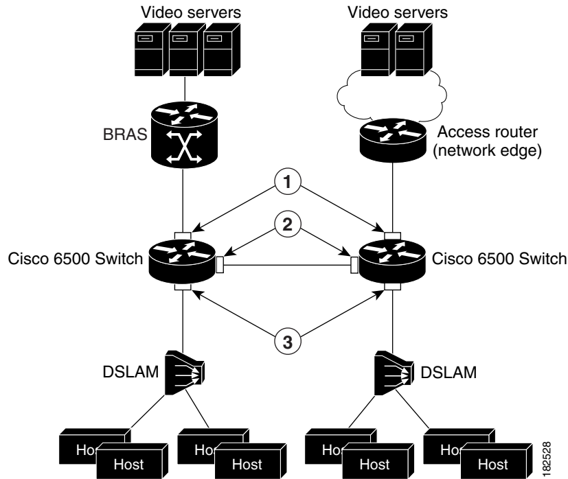
Figure 20-2 Private Hosts Port Types (Modes)
