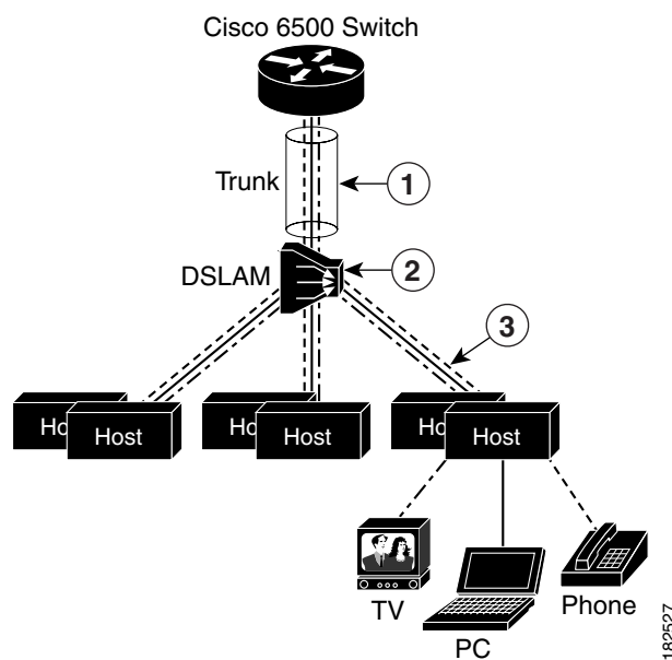
Figure 20-1 VC to VLAN Mapping
