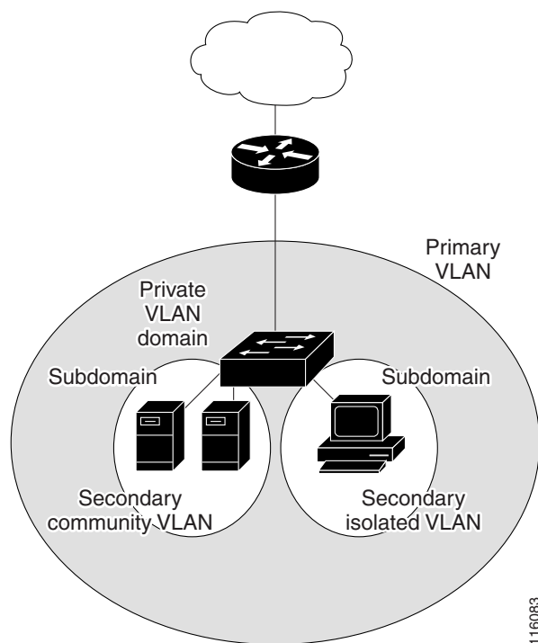
Figure 19-1 Private VLAN Domain
