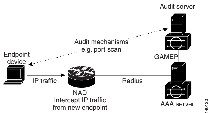
Figure 51-3 NAC Device Roles
