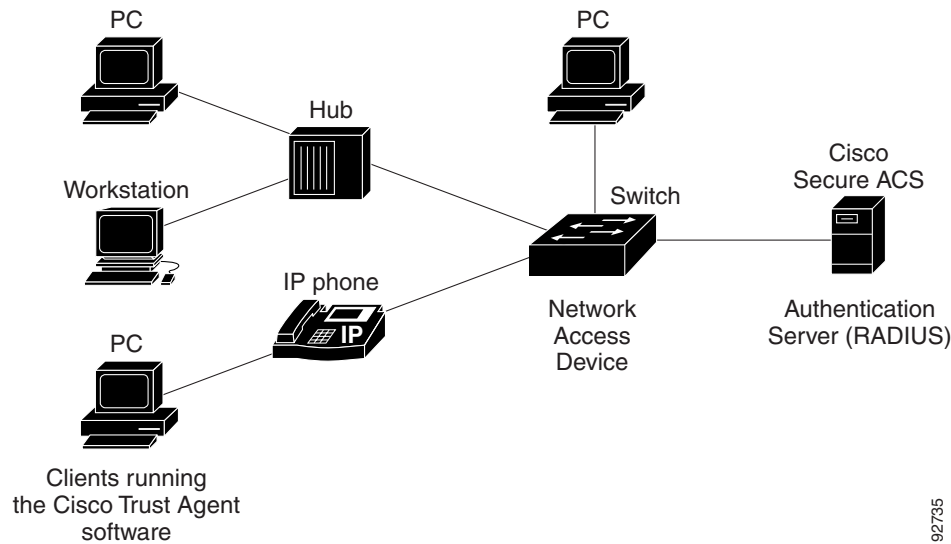
Figure 51-2 Network Using NAC Layer 2 IP
