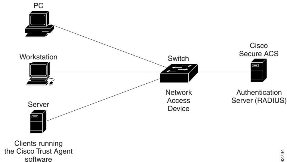
Figure 51-1 Posture Validation Devices
