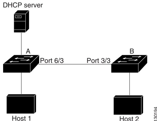
Figure 48-2 ARP Packet Validation on a VLAN Enabled for DAI
