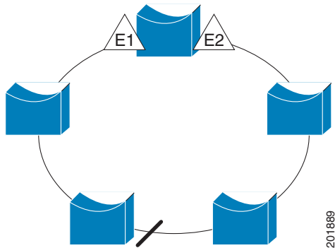
Figure 19-2 REP Ring Segment
