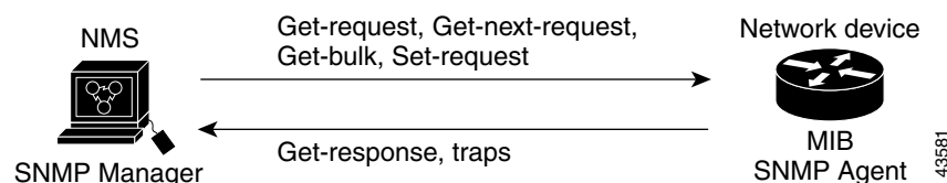
Figure 47-1 SNMP Network
