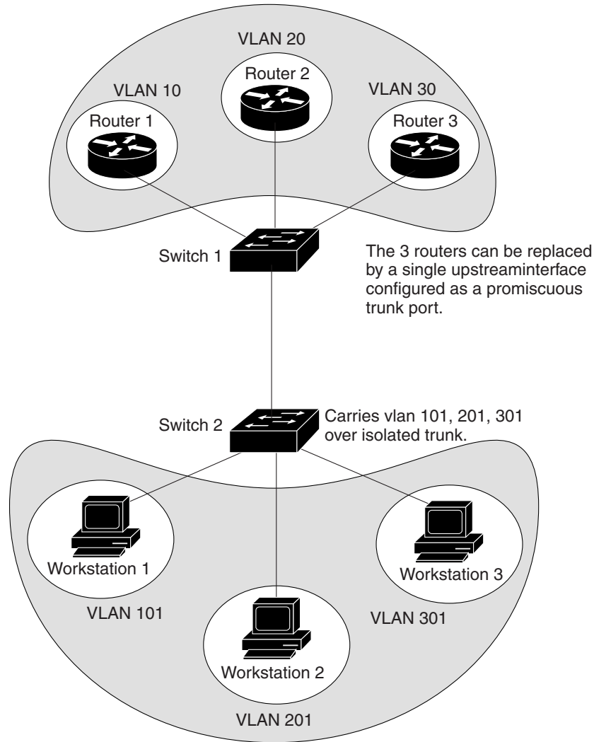
Figure 38-3 Private VLAN Trunk Topology
