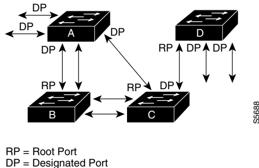
Figure 15-1 Spanning Tree Topology
