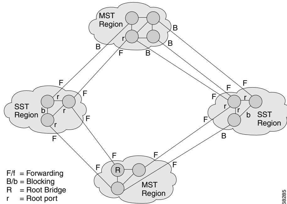
Figure 15-2 Network with Interconnected SST and MST Regions
