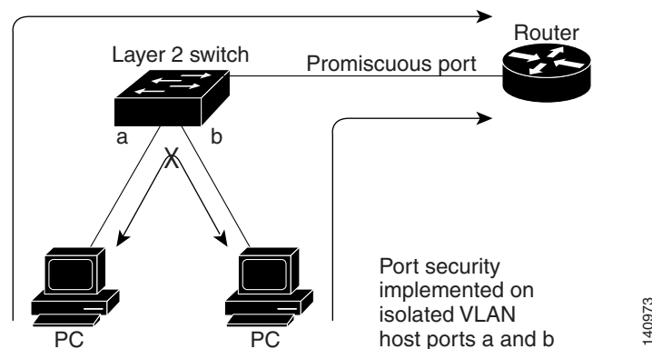
Figure 31-1 Port Security on Isolated Private VLAN Host Ports
