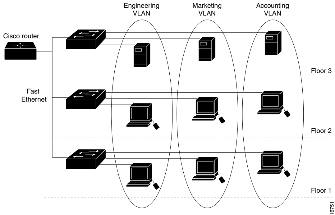
Figure 8-1 Sample VLANs
