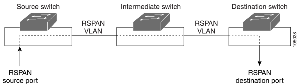
Figure 38-2 Example of RSPAN Configuration
