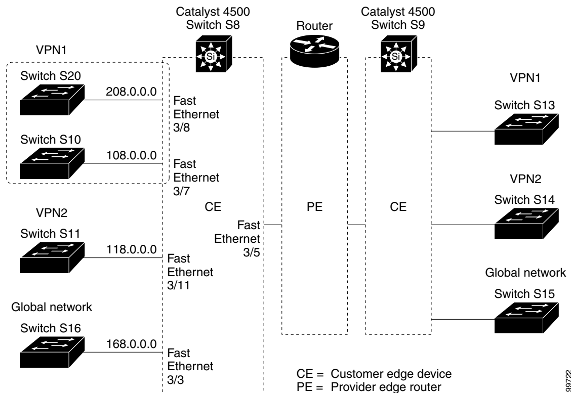
Figure 25-2 VRF-lite Configuration Example
