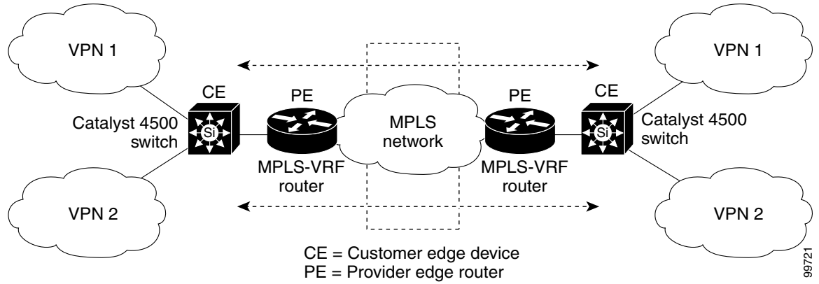
Figure 25-1 Catalyst 4500 Switches Acting as Multiple Virtual CEs
