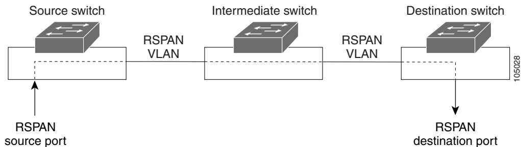
Figure 37-2 Example of RSPAN Configuration
