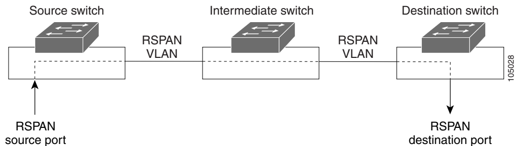
Figure 34-2 Example of RSPAN Configuration
