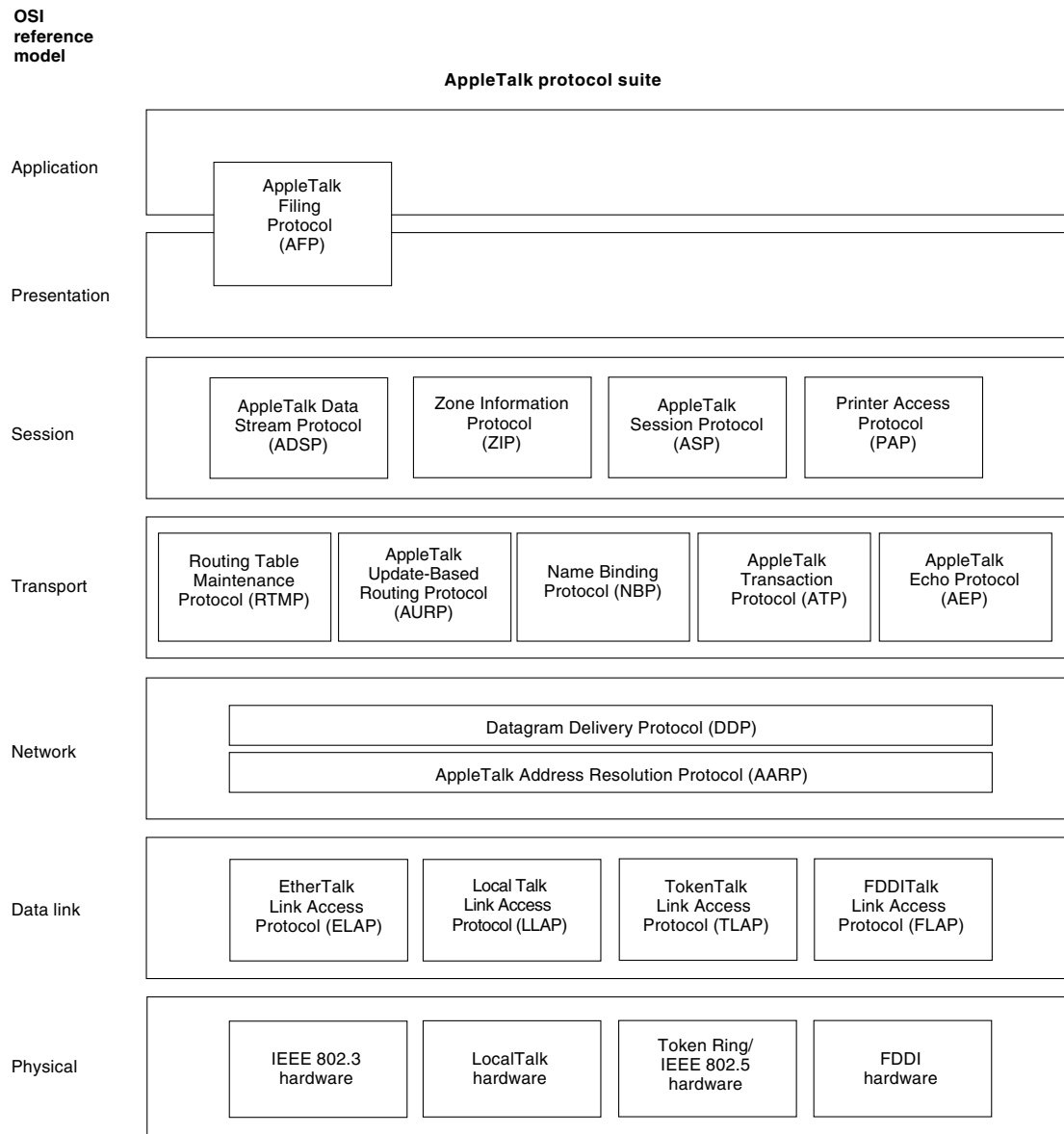
Figure 35-12 The AppleTalk Protocol Suite Maps to Every Layer of the OSI Model
