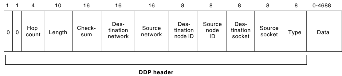
Figure 35-13 An Extended DDP Packet Consists of 13 Fields
