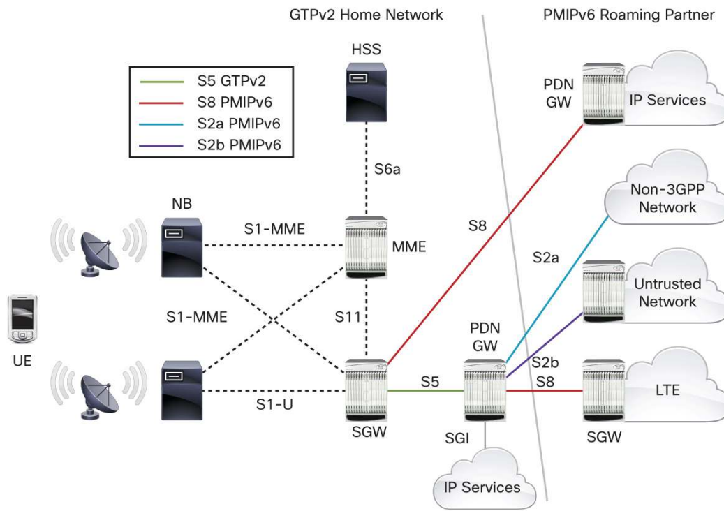
Figure 7. Roaming Support Between GTPv2 Home Network and PMIPv6-Based Roaming Partner
