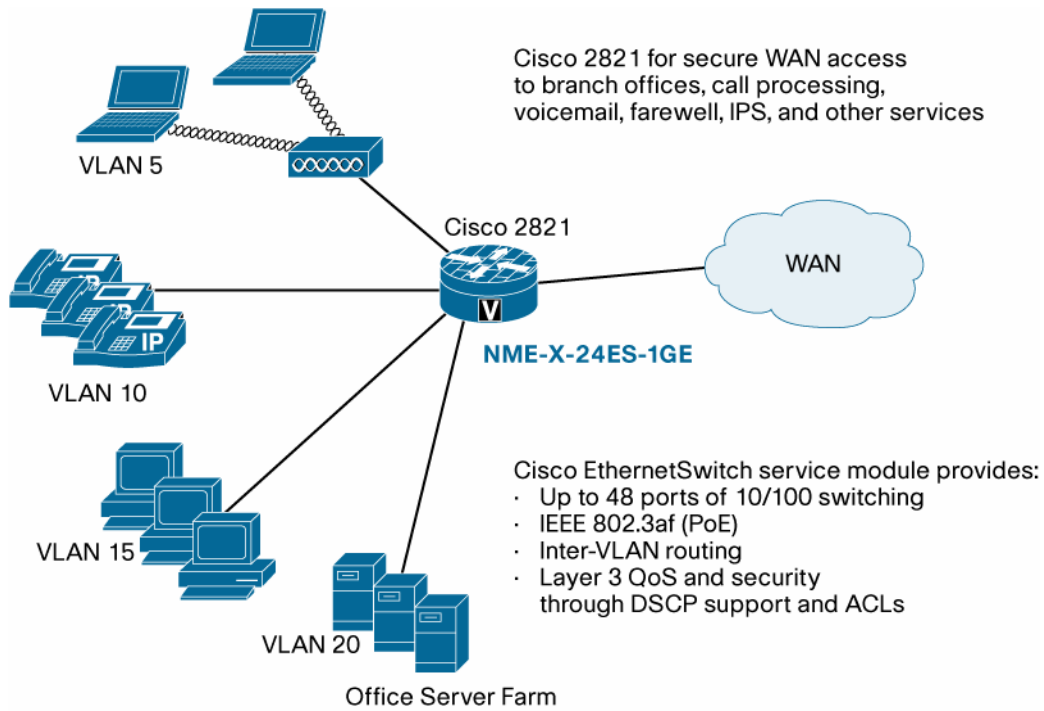
Figure 2. Cisco EtherSwitch Service Module with a Cisco 2821 Integrated Services Router
