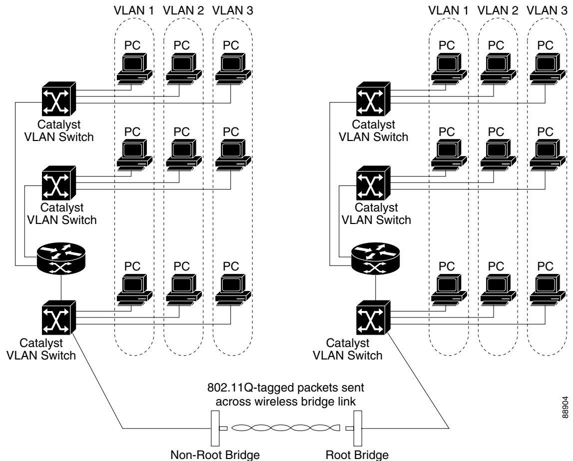
Figure 1 Bridges Connecting LAN Segments Using VLANs
