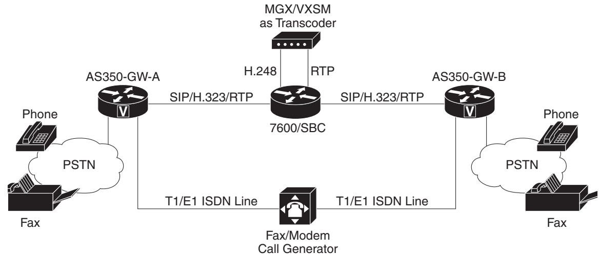
Figure 14-1 Transcoding Configuration
