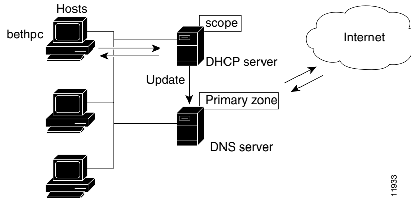
Figure 18-6 DNS Update at ExampleCo Company
