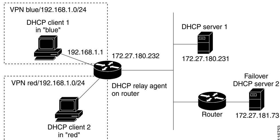
Figure 18-4 Virtual Private Network DHCP Configuration
