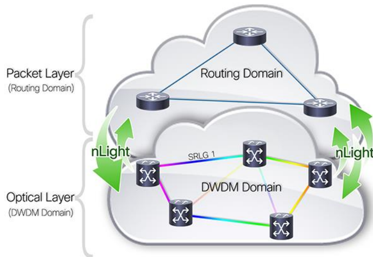
Figure 3. Cisco nLight Provides Benefits of Peering with Intelligent Information Sharing
